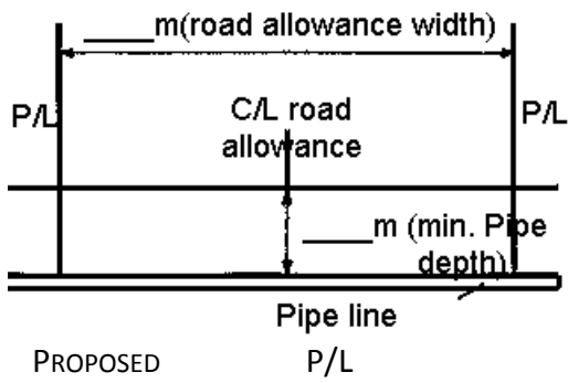
1. TYPICAL UNDEVELOPED ROAD ALLOWANCE (NOT TO SCALE)
