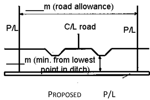
2. TYPICAL DEVELOPED ROAD ALLOWANCE (NOT TO SCALE)
